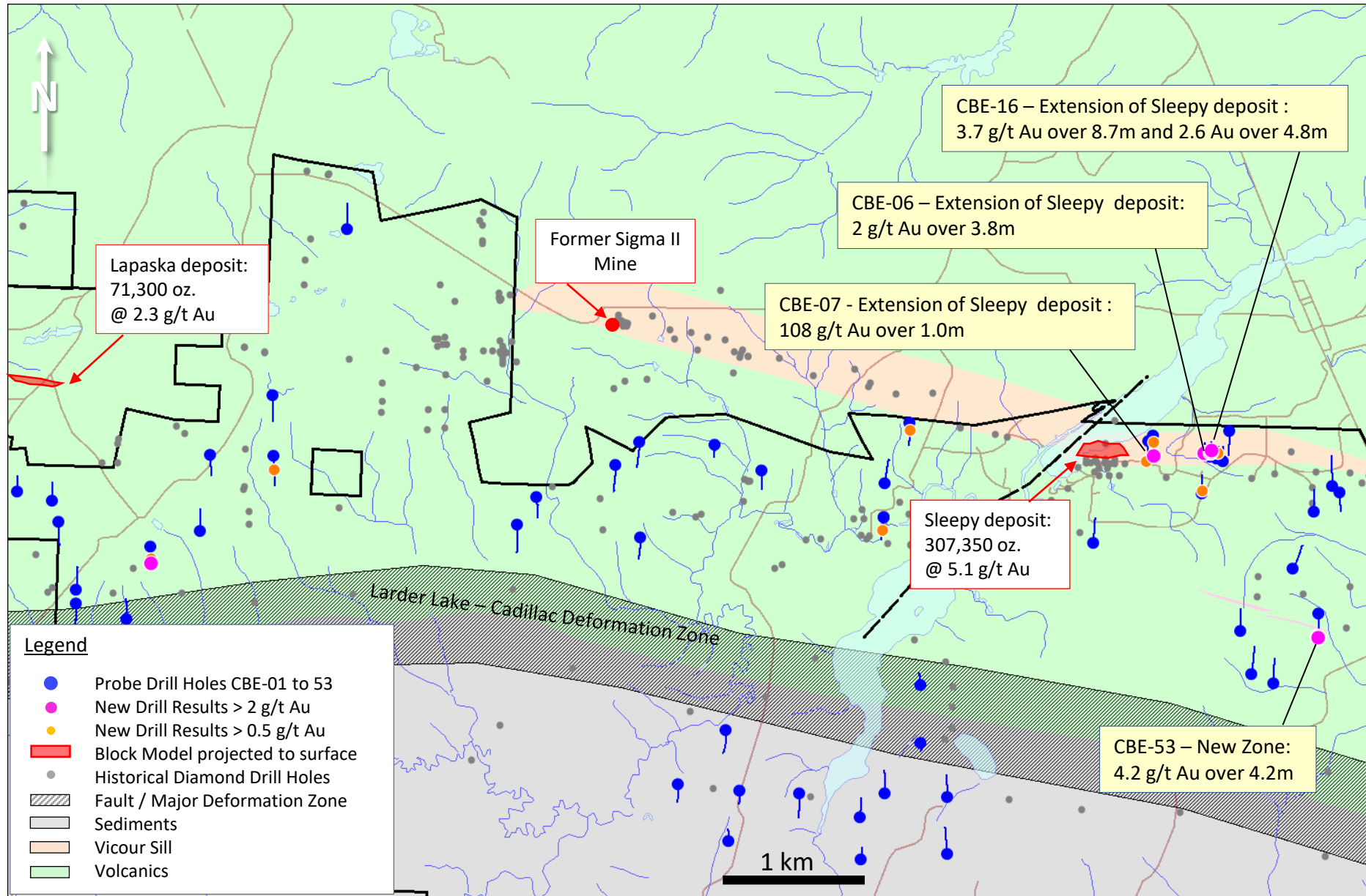
Figure 1: Surface Map – Cadillac Break East Drilling Results, June 2020
